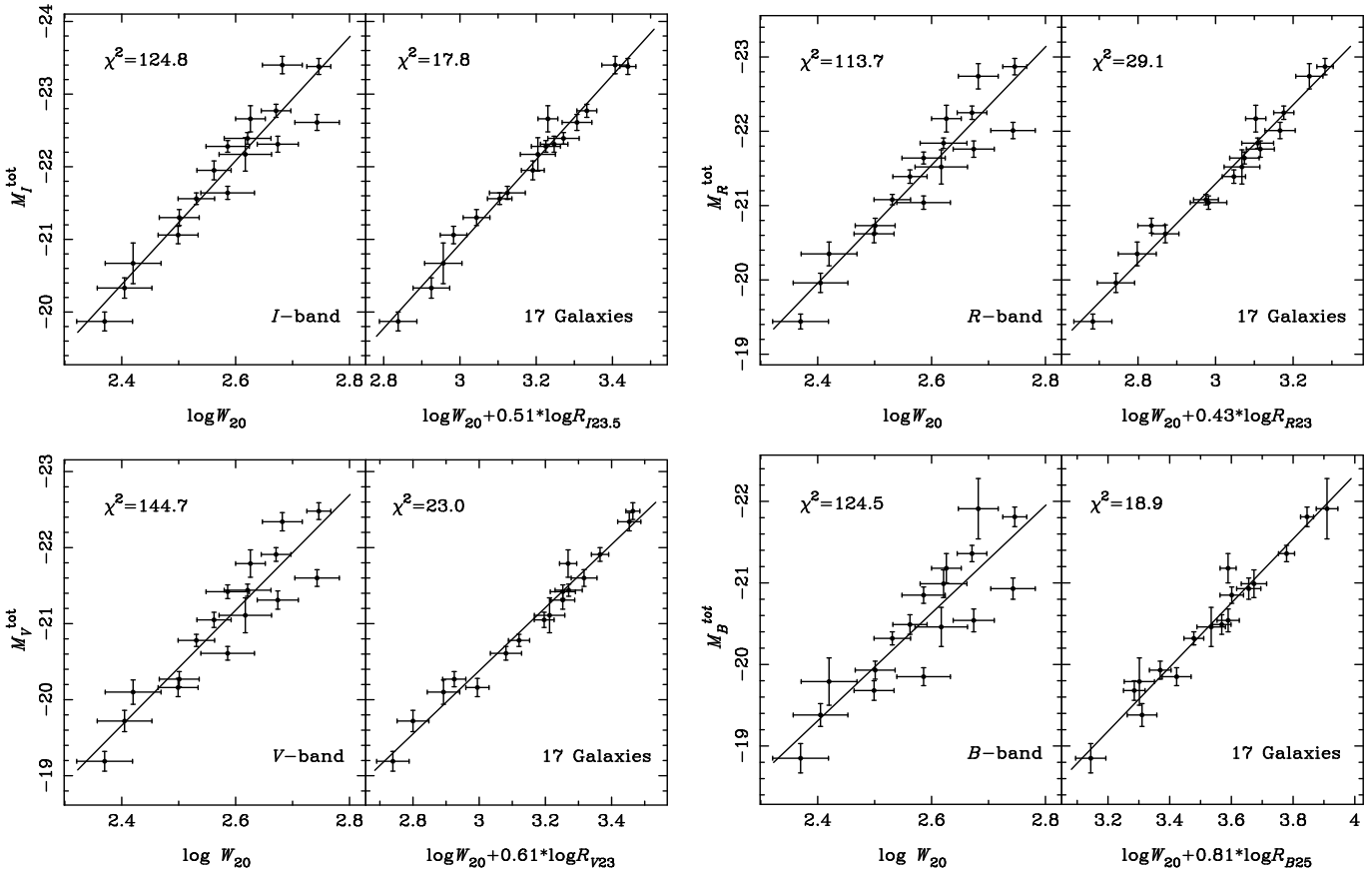
Fig. 2. Scattering from the Tully–Fisher relation (left) and the best-fitting plane (right) for the Hubble calibration galaxies at the IRVB bands. Data were taken from Sakai et al. (2000) and Macri et al. (2000).
